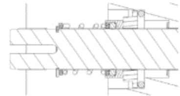
Shaft Seal Assembly – KIT700SL
