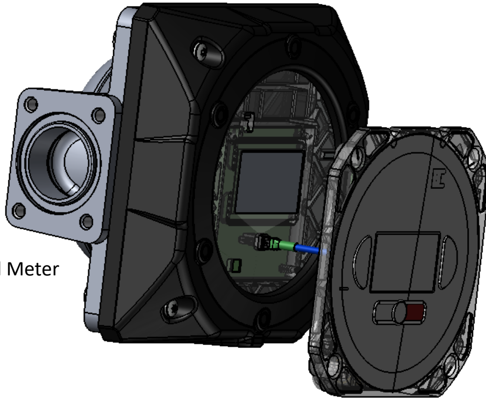
Register Assembly
